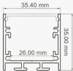
Profile Dimension
