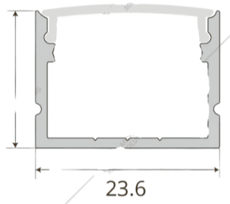
Profile Dimension
