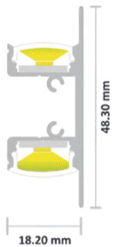
Profile Dimension
