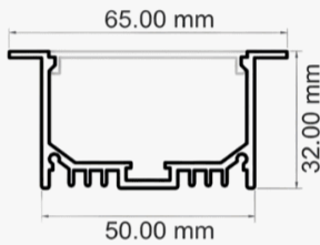
Cross-Section/ Dimension
