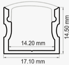
Profile Dimension
