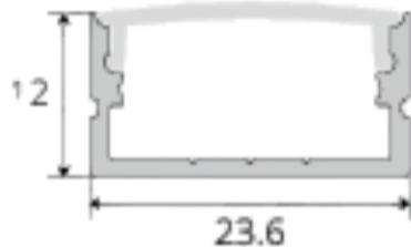
Profile Dimension
