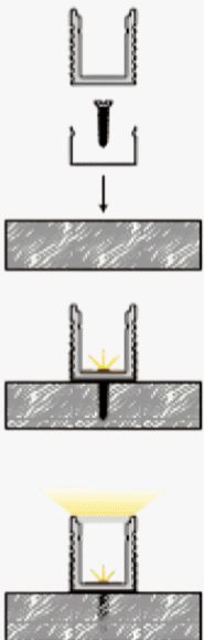
Installation Guide
